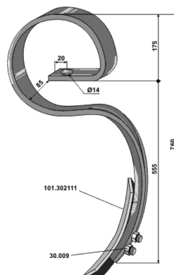
Dents Herkules 70x12
